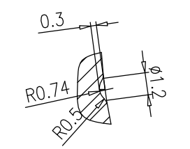
POINT SECTION 5:1
