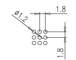
POINT SECTION 5:1
